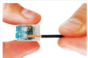
Strip conductor to 10mm Fio descarnado até 10mm Cable conductor de hasta 10mm
